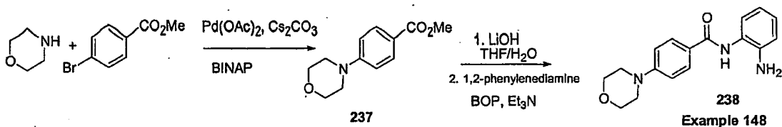
Scheme 37
